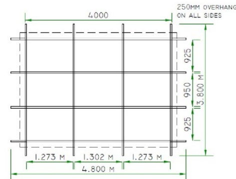
ROOF STRUCTURE
