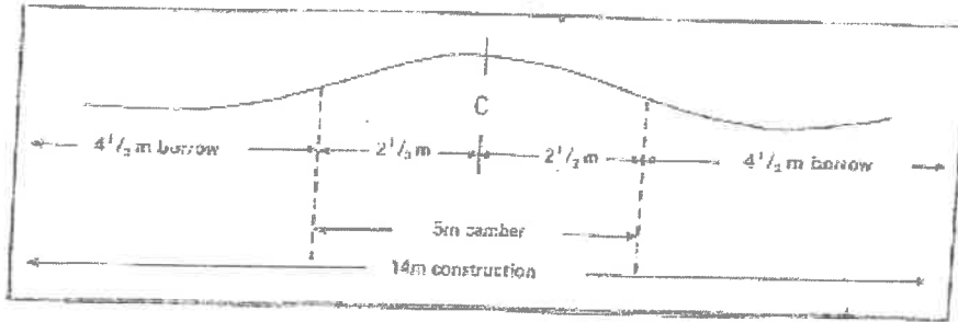
CROSS SECTION OF CREST ROAD
