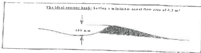
CROSS SECTION OF BROAD BASED CONTOUR BANK
