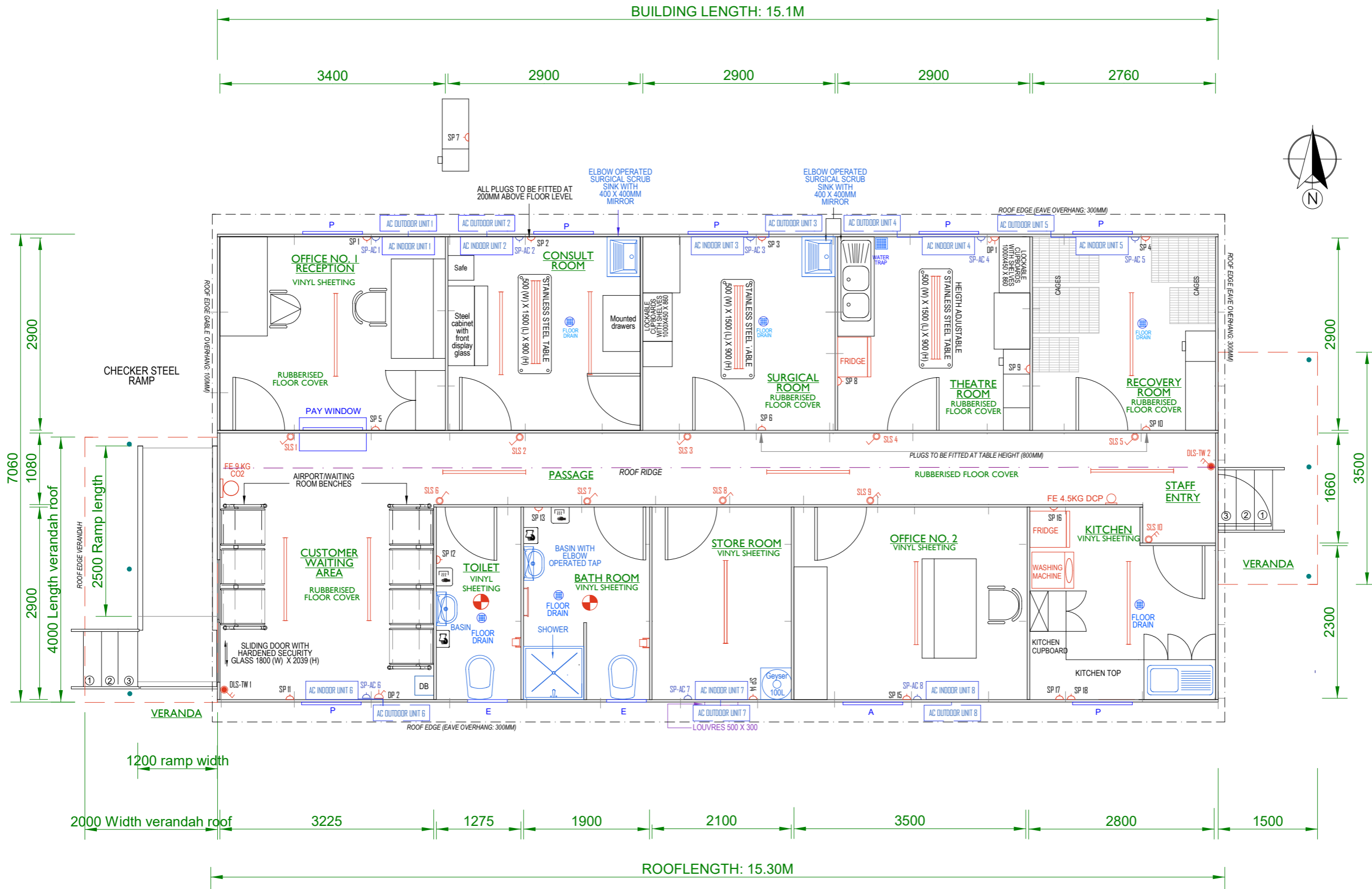
FLOOR PLAN
