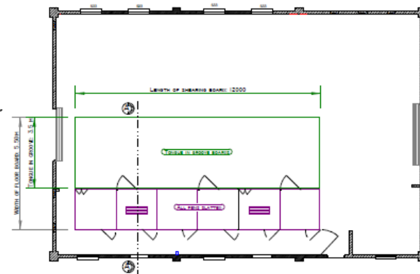
LOCATION OF FLOOR BOARD IN THE SHED
