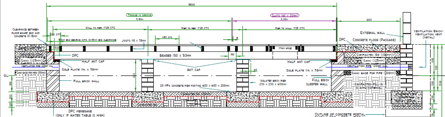
CROSS SECTION A-A :FLOOR BOARD, PEN SLATS AND PASSAGE
