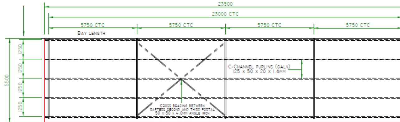
TOP VIEW SHOWING PORTALS, PURLINS & BRACING
