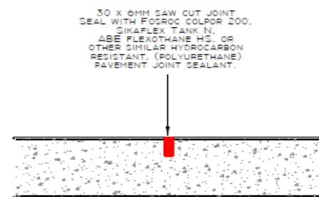
SAW CUT DETAIL
