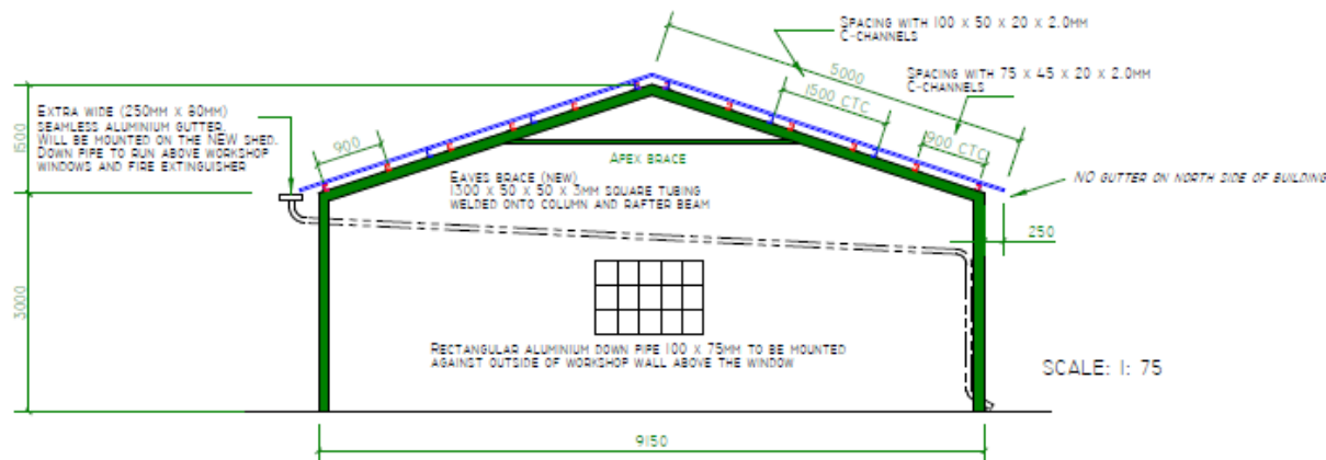
EXISTING SHED - PORTAL
