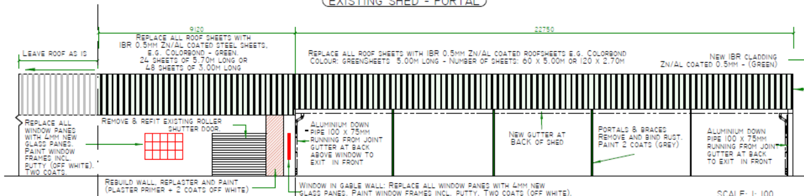
EXISTING SHED - PORTAL
