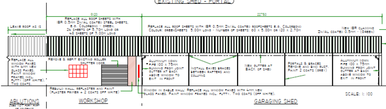
ELEVATION OF EXISTING GARAGING SHED SHOWING SCOPE OF WORKS FOR REFURBISHMENT
