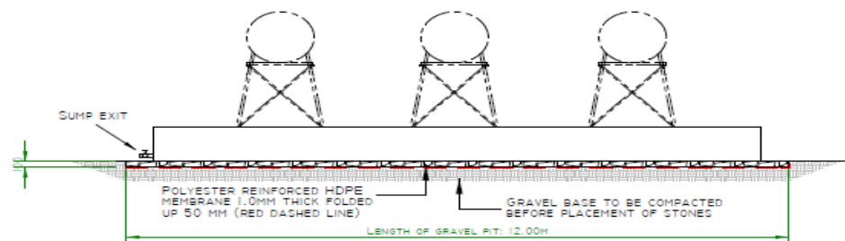
CROSS SECTION FILLING AREA
