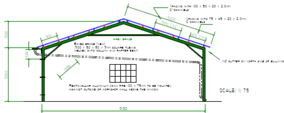
EXISTING SHED - PORTAL
