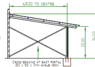
WEST ELEVATION
