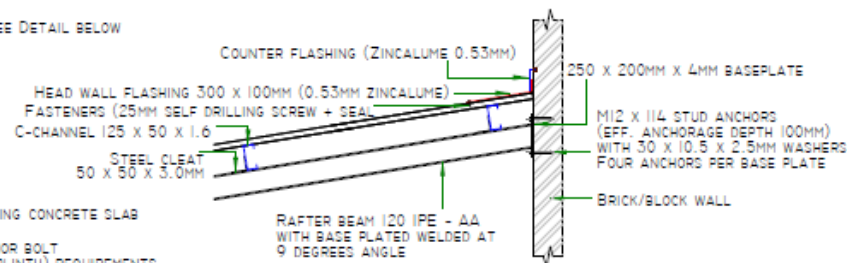
ROOF DETAIL SHOWING HEAD WALL FLASHING
