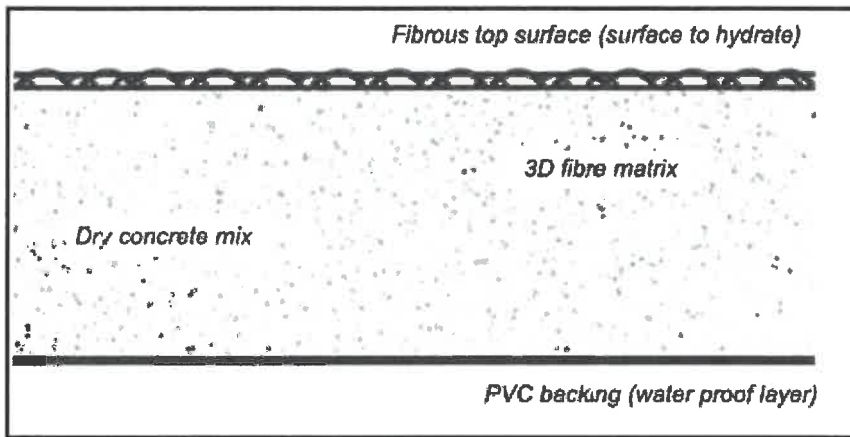
Figure 0.2 Typical concrete impregnated fabric installation
