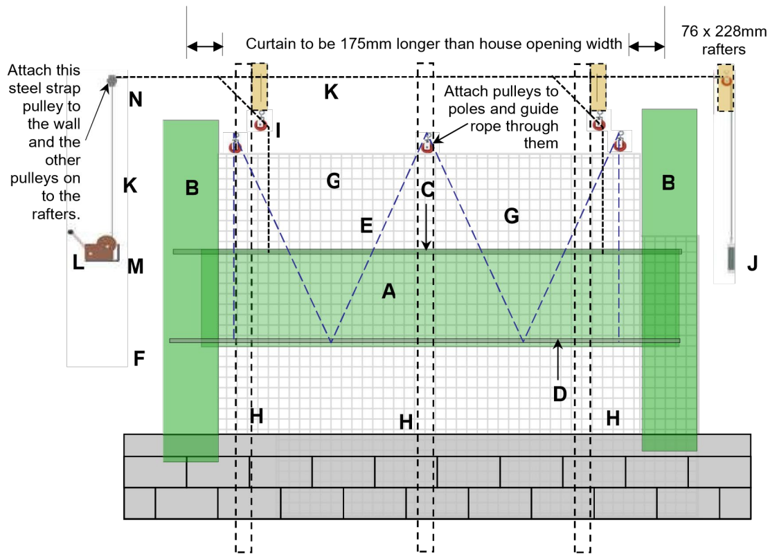
Figure 4: Diagram showing the various elements of the PVC Curtains
