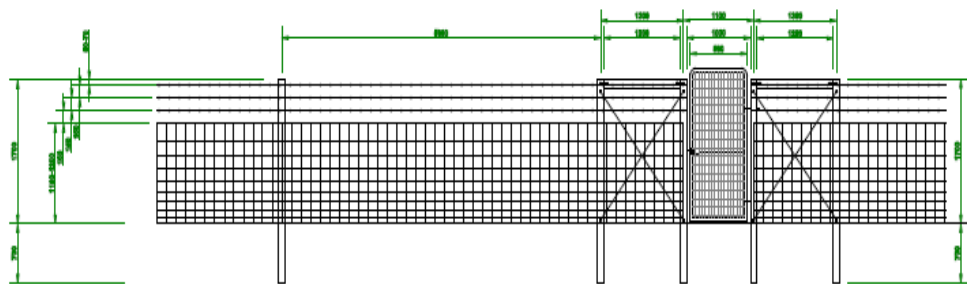
FENCE LINE WITH PEDESTRIAN GATE
