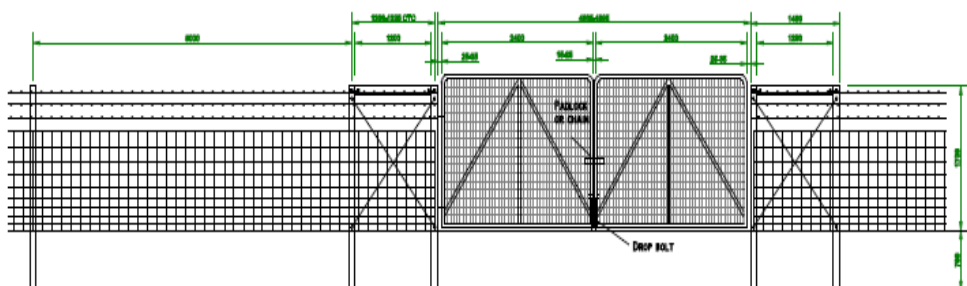
FENCE LINE WITH DOUBLE TRACTOR GATE
