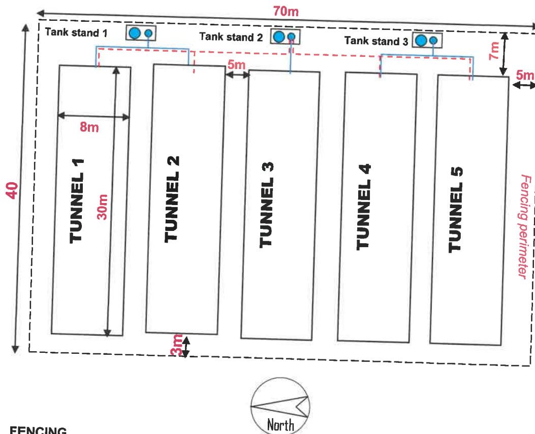
Figure 1: Site plan showing the 5 tunnels and location of the tank stands.
