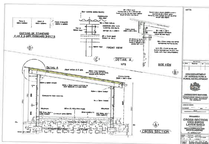
Figure 1: Cross section showing floor & floor base, timber frame & installation details for isoboard insulation Please note that the corrugated iron cladding should in fact be a curtain, as shown on the attached Drawing 4 : RDN/2016/030/ANS
