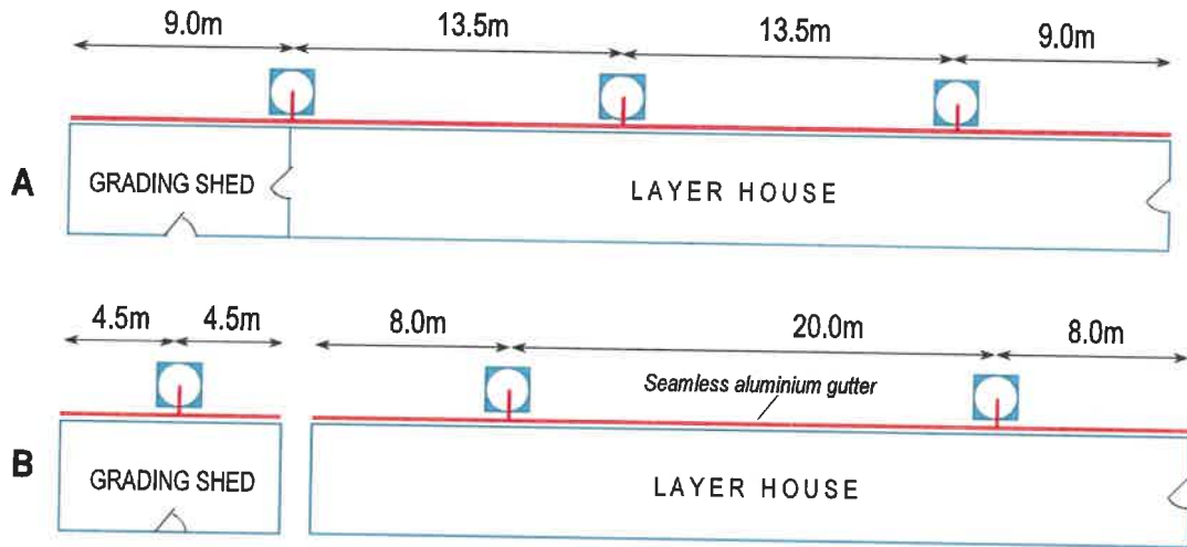
Figure 10: Location of water tanks in case grading shed is built onto layer house (A) and when separate (B).
