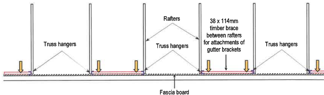
Figure 2: Gutter connection points to roof structure (Top view)
