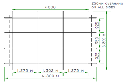
ROOF STRUCTURE
