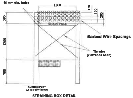
STRAINING BOX DETAIL
